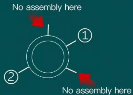
Drawing of two-claw assembly
